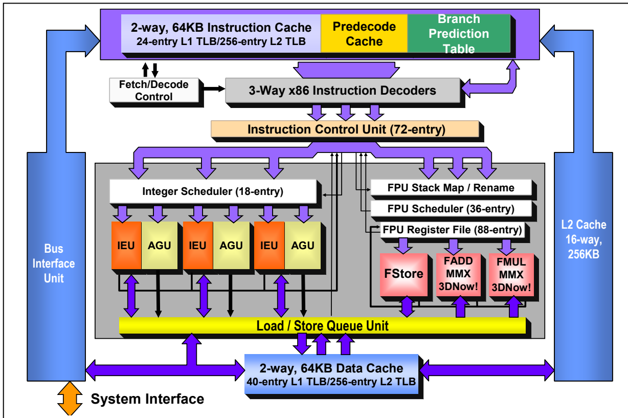
Figure 1: Mobile AMD Athlon™ XP Microarchitecture Block Diagram.
